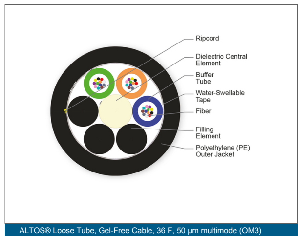
ALTOS® Loose Tube, Gel-Free Cable, 36 F, 50 µm multimode (OM3)
