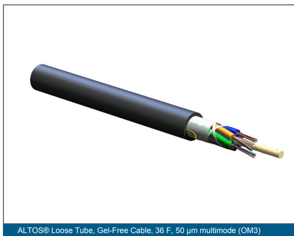
ALTOS® Loose Tube, Gel-Free Cable, 36 F, 50 µm multimode (OM3)
